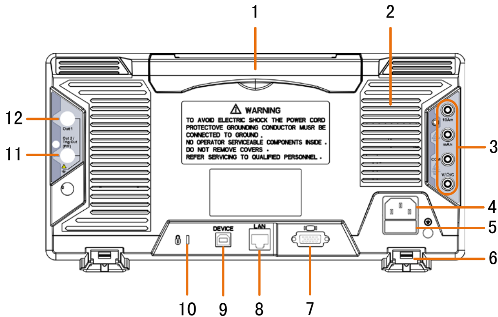
Figure 3-2 Rear Panel
