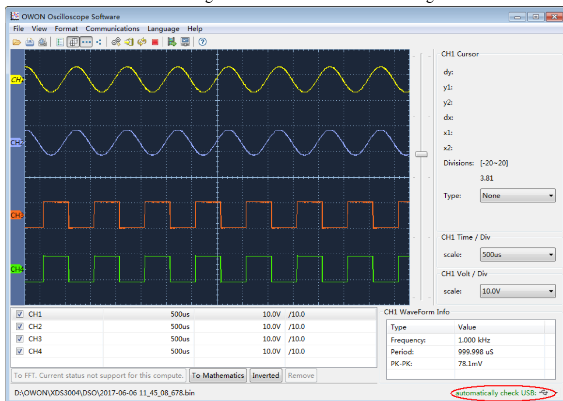
Figure 7-1 Connect with PC through USB port
