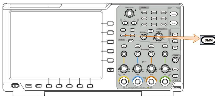
Figure 6-2 Multimeter Button
