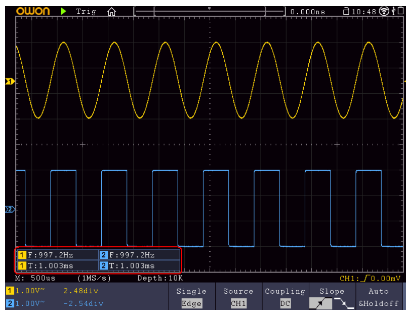
Figure 4-13 Automatic measurement
